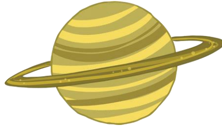
Saturn
